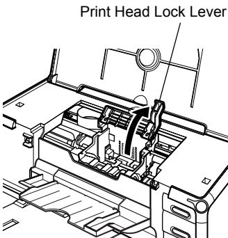
Print Head Lock Lever
